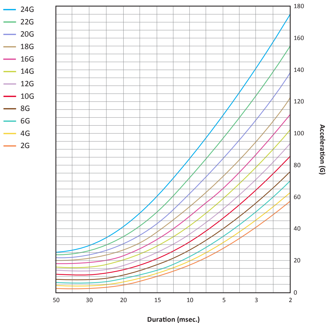
MAG 2000 Activation Acceleration vs. Duration (Even Values, 2G thru 24G)
